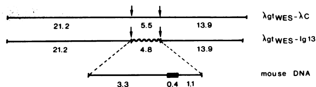
FIG. 4. Schematic representation of the maps of \lambda\text{gt}_{\text{WES}} - \lambda\text{C} and \lambda\text{gt}_{\text{WES}} -Ig 13. The arrows point to EcoRI cleavage sites. All lengths are given in kilobase (kb) units. The boxed area in the mouse DNA insert represents the region of sequence homology with HOPC 2020 mRNA.
