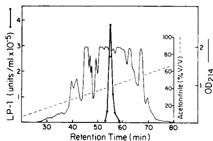
FIGURE 5. First-phase purification of LP-1 by RP-HPLC. The active fractions from a typical Blue B chromatography purification were applied to a C 4 column and eluted with increasing concentrations of acetonitrile in 0.1% TFA.
