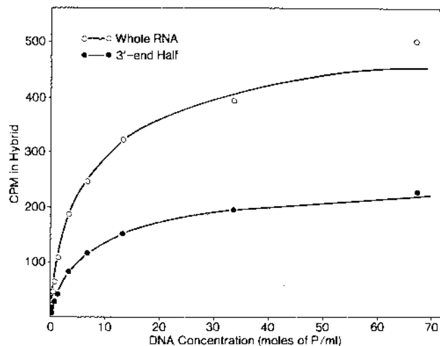
FIG. 1. Dependency of hybridization level on DNA concentration. ^{125}\text{I} -Labeled, whole \kappa mRNA of MOPC 321 (1300 cpm) or its 3'-end half fragment (600 cpm) was annealed with varying indicated amounts of denatured MOPC321 DNA in 0.3 M NaCl, 0.03 M sodium citrate (pH 7) at 70^\circ for 42 hr. The volume of annealing mixture was 0.05 ml. Specific activity of the RNA was 6.5 \times 10^7 cpm/ \mu\text{g} . Each point represents an average of duplicate measurement. Intrinsic RNase-resistant counts, 22 cpm for whole RNA and 16 cpm for 3'-end half, are subtracted.
