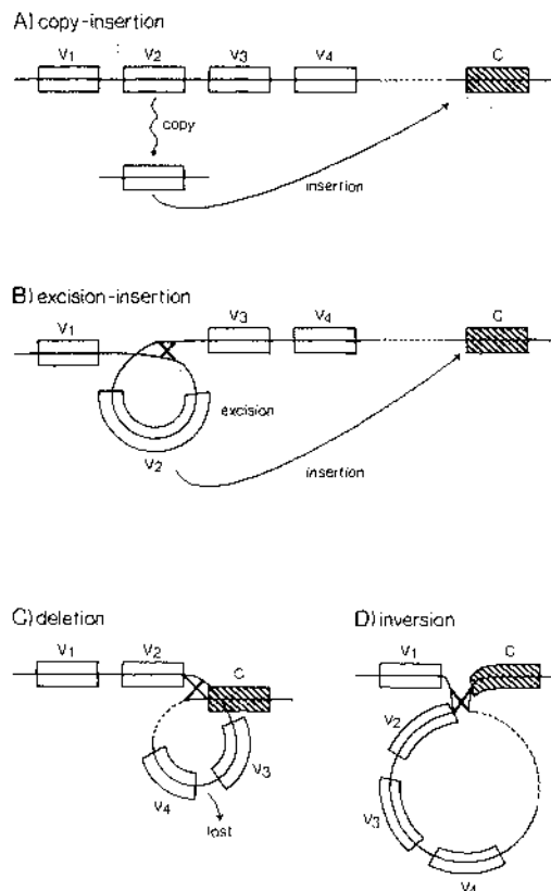
FIG. 4. Models for V-C gene joining at DNA level. See text for explanation.
