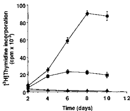
Fig. 1. Anti-CD40-induced proliferation of normal B lymphocytes is long lasting and enhanced by IL-4. Purified spleen B cells ( 2.5 \times 10^5 , >97% CD20 + ) were cultured in flat-bottom microwells for up to 10 days on 2.5 \times 10^3 irradiated CDw32 L cells without MAb 89, without IL-4 (□); without MAb 89, with IL-4 (100 U/ml) (▲); with MAb 89, without IL-4 (■); with MAb 89, with IL-4 (100 U/ml) (●). IL-4 is a purified recombinant protein (specific activity, 10^7 U/mg) obtained from Schering-Plough Research. [ ^3 H]Thymidine pulses (16 hours) were performed daily. Results are means \pm SD of triplicates.
